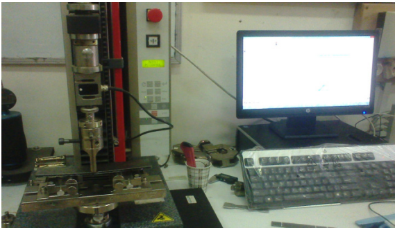
Fig. 13. Photography of the three-point bending test machine
