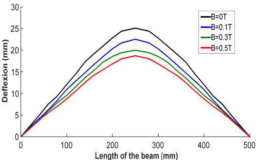
Fig. 15. Deflection obtained by experimental analysis for different values of the magnetic field
