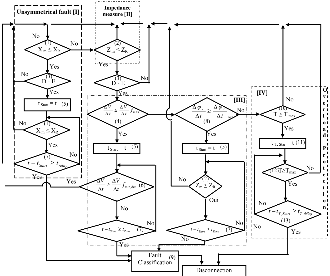
Fig. 5 Distance Relay Scheme used during abnormal operating conditions
