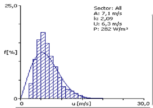
Fig. 2. Wind Speeds distribution (2003-2008) [6]
