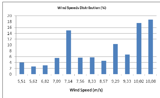
Fig. 4. Site Wind speed distribution (50m height)
