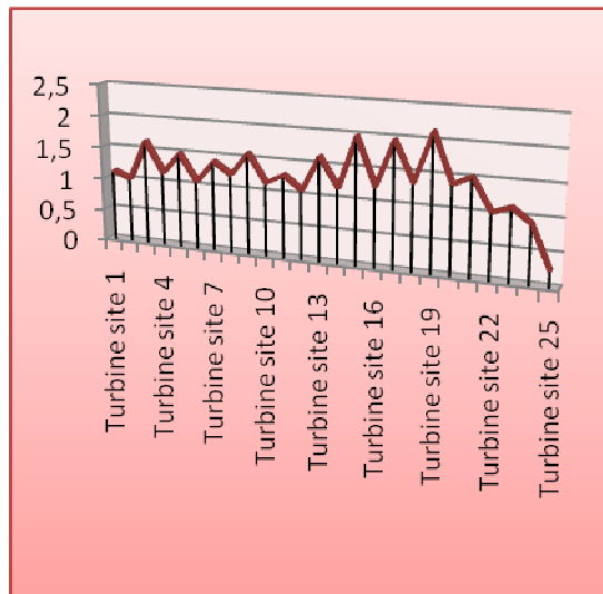
Fig. 8. Wake loss Variation for each turbine
