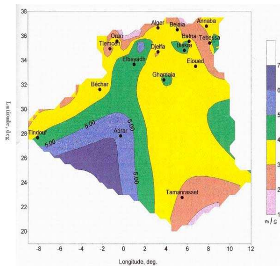
Fig. 1. Wind Chart of Algeria [5]
