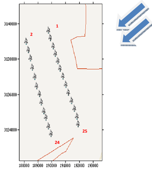
Fig. 9. Third Wind Farm layout
