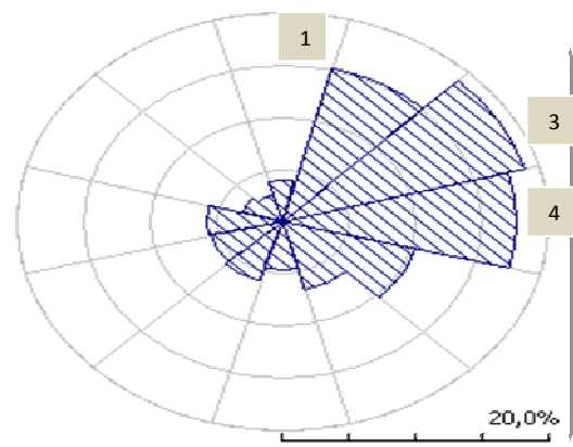
Fig. 2. Wind Speeds distribution (2003-2008) [6]
