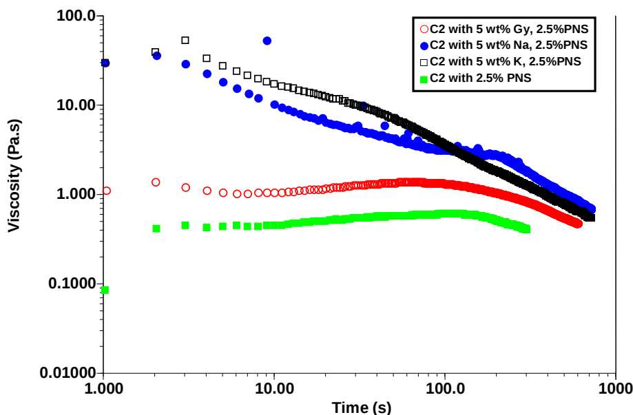
Figure 15. Time dependent behavior of paste C2 (C2, C2- \text{Ca}^{2+} , C2- \text{Na}^+ and C2- \text{K}^+ ).
