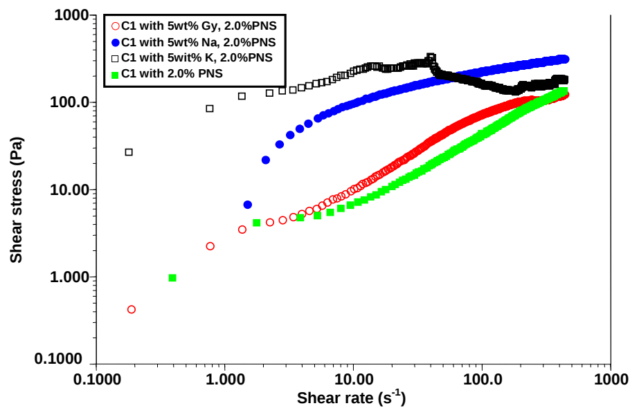
Figure 10. Shear stress as a function of shear rate of cement pastes (C1, C1- \text{Ca}^{2+} , C1- \text{Na}^{+} and C1- \text{K}^{+} ) after 12 min of hydration W/C=0.3, with PNS.
