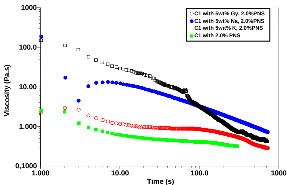
Figure 12. Time dependent behavior of paste C1 (C1, C1- \text{Ca}^{2+} , C1- \text{Na}^{+} and C1- \text{K}^{+} ).
