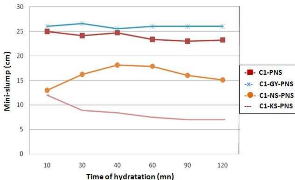
Figure 8. Fluidity and mini-slump tests as a function of hydration time of cement paste C1 (C1- \text{Ca}^{2+} , C1- \text{Na}^+ and C1- \text{K}^+ ) for a W/C = 0.30, with 2% of PNS.
