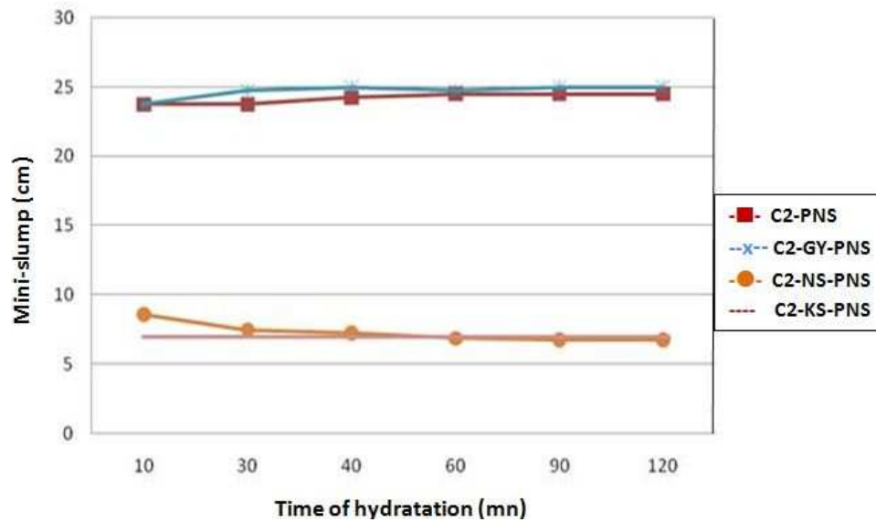
Figure 9. Fluidity and mini-slump tests as a function of hydration time of cement paste C2 (C2- \text{Ca}^{2+} , C2- \text{Na}^{+} and C2- \text{K}^{+} ) for a W/C = 0.30, with 2.5% of PNS.
