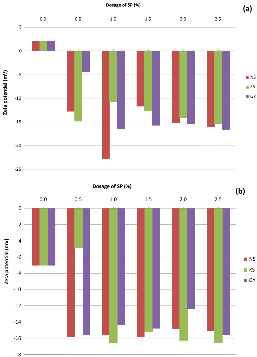
Figure 16. Variation of zeta potential in cement pastes with increase of PNS; (a) C1 (b) C2.
