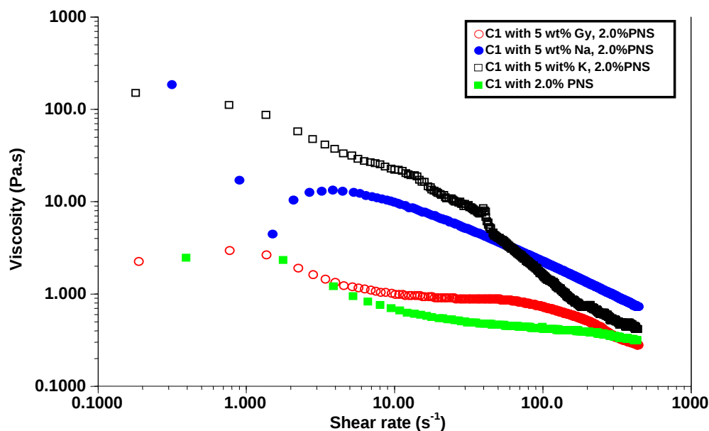
Figure 11. Apparent Viscosity as a function of shear rate of cement pastes (C1, C1- \text{Ca}^{2+} , C1- \text{Na}^{+} and C1- \text{K}^{+} ) after 12 min of hydration W/C=0.3, with PNS.
