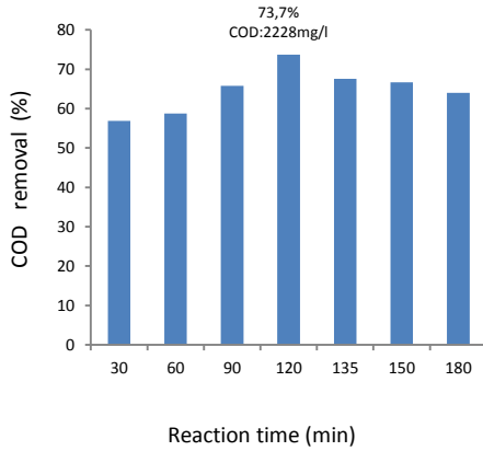
Figure 7. Effect of reaction time on COD removal efficiency (conditions: initial pH= 3.5; H 2 O 2 = 5g/l; H 2 O 2 /Fe (II) molar ratio=6, original COD=8474.7 mg/l)
