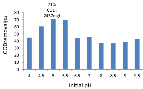
Figure 3. Effect of initial pH on COD removal efficiency ( \text{FeCl}_3=1.6\text{g/l} ; original COD 8474.72 mg/l)
