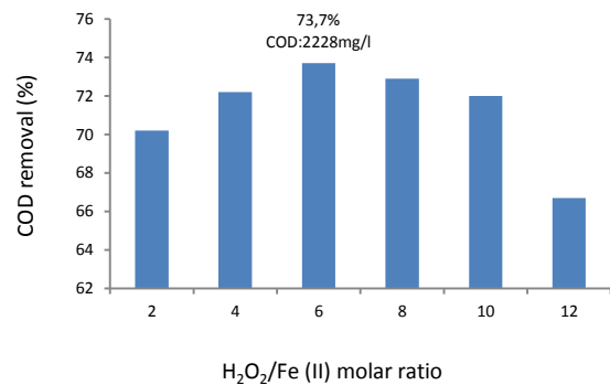
Figure 4. Effect of \text{H}_2\text{O}_2 / \text{Fe}(\text{II}) molar ratio on COD removal efficiency (conditions: initial pH= 3; \text{H}_2\text{O}_2= 5\text{g/l} ; original COD=8474.7 mg/l)
