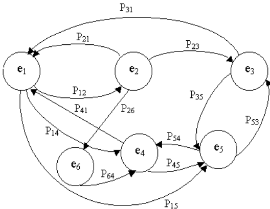
Fig. 7 Semi-Markovian process states and transitions graph
