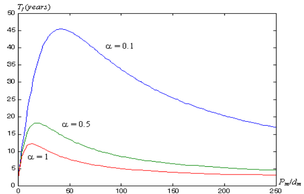
Fig. 8 mean time between failures variation according to ration Pm/dm .
