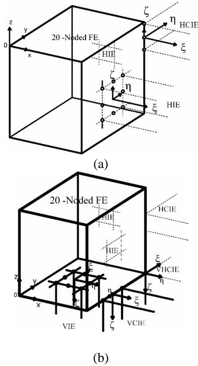
Fig. 3 Geometrical mappings: (a) Horizontal layered region; (b) Underlying halfspace
