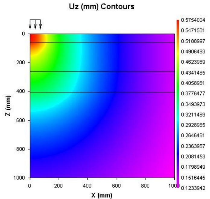
Fig. 10 Contour plot of vertical displacement
