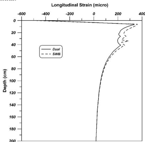
Fig. 8 Variation of the longitudinal strain ( \epsilon_{xx} ) with depth
