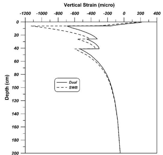
Fig. 9 Variation of the vertical strain ( \epsilon_{zz} ) with depth
