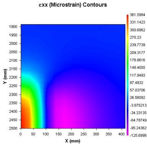
Fig. 11a Tensile strain at a bottom of asphalt layer
