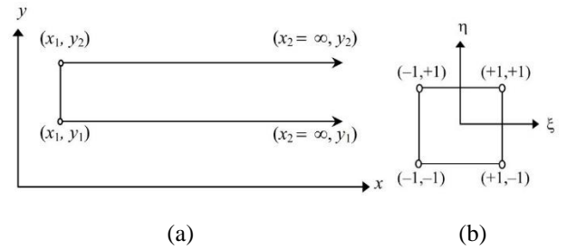
Fig. 2 Mapped infinite element in the horizontal direction: (a) physical co-ordinates, (b) local co-ordinates
