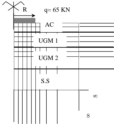
Fig. 5 Analysed pavement structure
