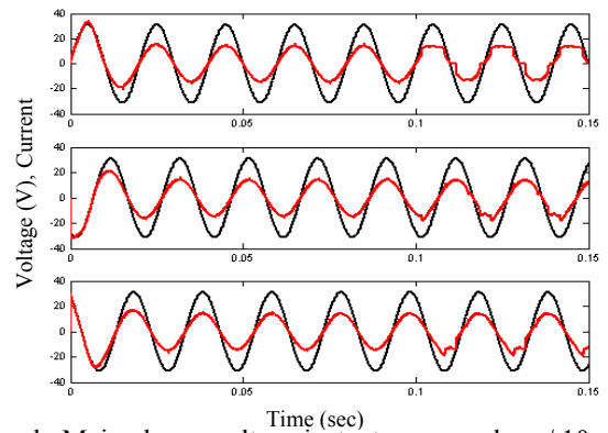
b. Main phases voltage instantaneous values / 10, main source phases currents instantaneous values before and after TR1 open fault condition
