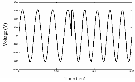
a. Main first phase voltage instantaneous values
