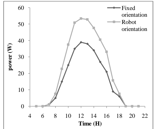
Fig. 6: The power variation of a photovoltaic module (spring)
