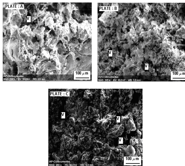
Fig. 1: Electron Micrographs of the bottom ashes obtained by incineration at different temperature from the leather waste shavings (V = bladders)
