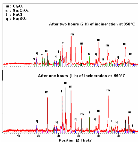
Fig. 3: XRD patterns of the bottom ash obtained after 1 and 2 hrs of incineration at 950°C from the leather waste shavings
