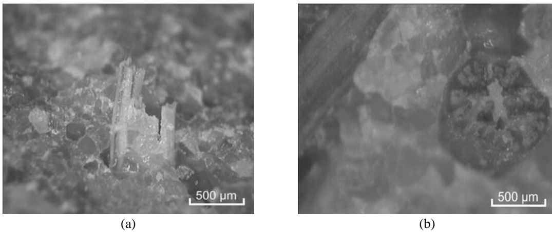
Fig. 6 Optical micrographs of PC fractured surfaces: (a) PC-0000-1%, and (b) PC-0524-1%
