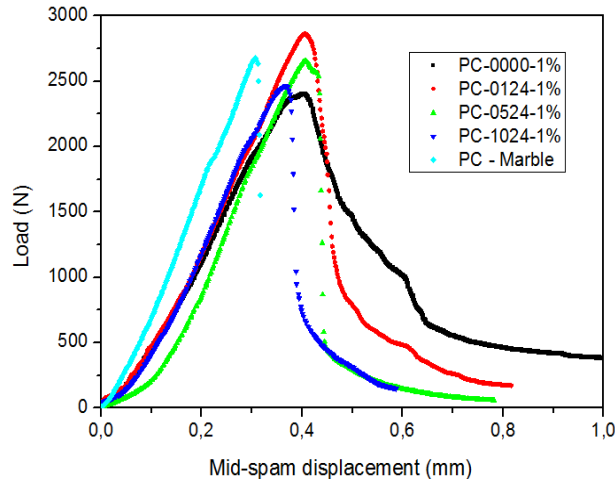
Fig. 4 Typical load vs. mid-span displacement test results of PC reinforced 1% Alfa fibers
