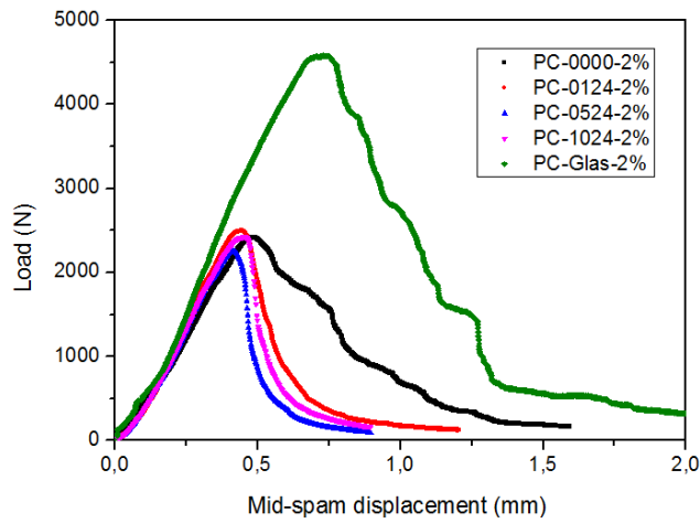
Fig. 5 Typical load vs. mid-span displacement test results of PC reinforced 2% Alfa fibers
