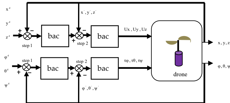
Figure 2. System block diagram.
