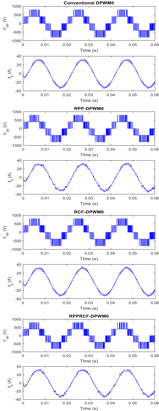
Fig. 6 – Simulated voltage (upper trace) and current (lower trace), ( f_s = 2 kHz, M = 0.8 , voltage: 500 V/div., current: 20 A/div.)
