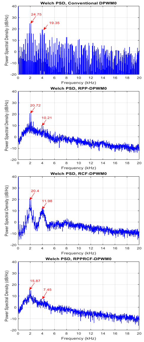
Fig. 7 – Welch PSD of phase-to-phase voltage, ( f_s = 2 kHz, f = 50 Hz, M = 0.8 , X-axis: 2 kHz/div., Y-axis: 10 dB/div.)
