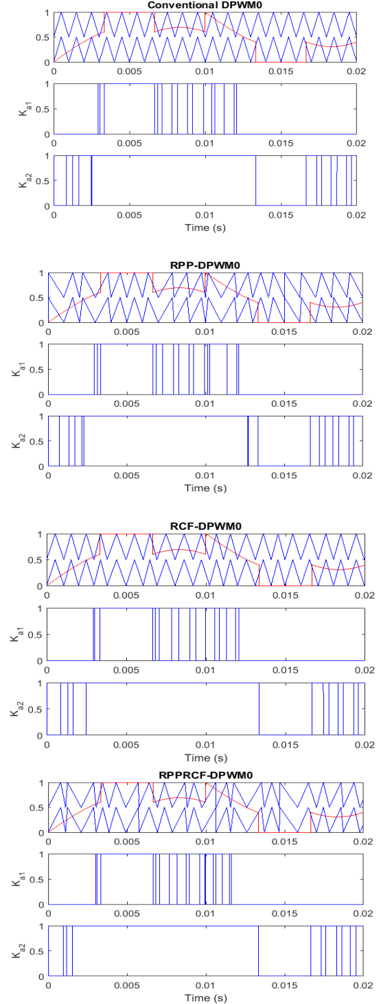
Fig. 5 – Simulated waveforms of triangular carrier and modulating function (upper trace), switching signal for K_{a1} (middle trace), switching signal K_{a2} (lower trace) ( f_s = 2 kHz, M = 0.8 , R_T = 0.2 , R_\beta = 1.2 ), (a) DPWM, (b) RPP-DPWM, (c) RCF-DPWM, (d) RPPRCF-DPWM.
