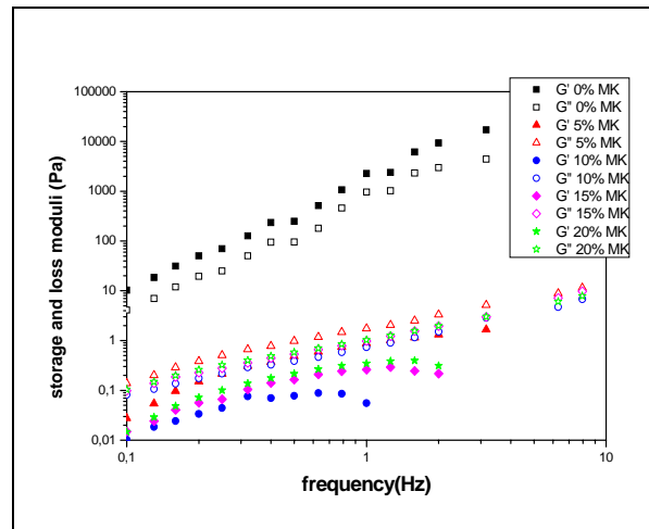
Figure 7: Storage and loss modulus as function as frequency of cement pastes for different proportion of MK
