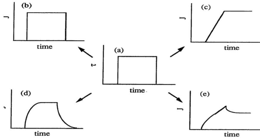
Figure 1: General creep/recovery behaviour of (b) elastic solid, (c) viscous liquid, (d) viscoelastic solid, (e) viscoelastic liquid under shear stress (a).
