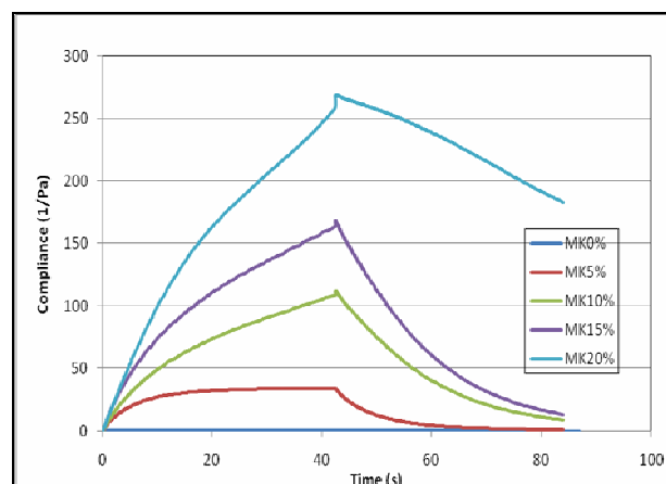
Figure 8: Creep /Recovery curves of MK cement pastes.
