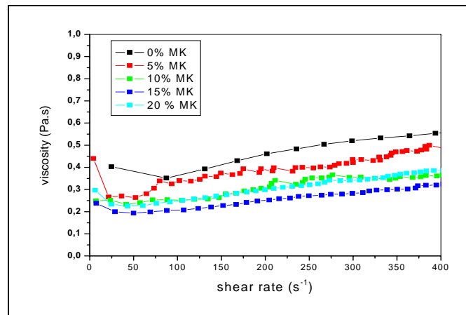
Figure 6: Evolution of viscosity of cement pastes for different proportion of MK.
