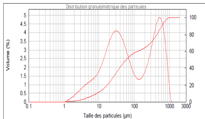
Figure 4: Particle size distribution of metakaolin
