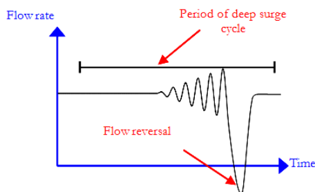
Fig. 3d: Deep surge of the flow rate
