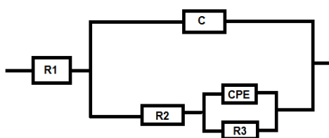
Figure 7. Electrical equivalent circuit of the positive plate electrode in 0.5 M H 2 SO 4
