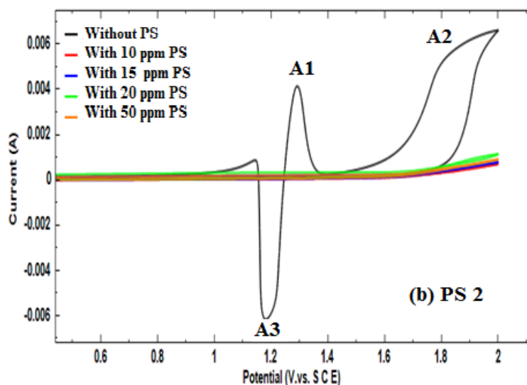
Figure 1. Cyclic voltammograms portion of pure Pb electrode in 0.5 M \text{H}_2\text{SO}_4 : (a) In the presence of PS N° 1; (b) in the presence of PS N° 2, at a scan rate 5 \text{ mVs}^{-1} .
