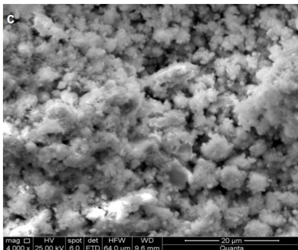
Figure 2. SEM imaging of \text{PbO}_2 after one cycle of charge/discharge in \text{H}_2\text{SO}_4 : (a) without PS, (b) with the presence of PS N°1 and (c) with the presence of PS N° 2.
