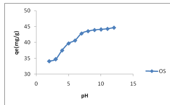
Fig.3: Effect of pH on the adsorption of methylene blue on the adsorbents in the native state ( C_i = 100 \text{ mg / l} , w = 150 \text{ rpm} , T^\circ = 20^\circ \text{ C} )
