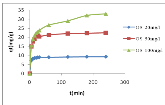
Fig 2: BM adsorption capacity by OS according to the time of contacts [ C_0 = 20, 50, 100 \text{ mg / l} ], \text{pH} = 5.6 , T^\circ = 20^\circ \text{ C} , w = 150 \text{ rpm} ].
