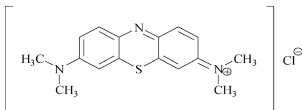
Fig 1: structure of the Methylene blue (MB)
