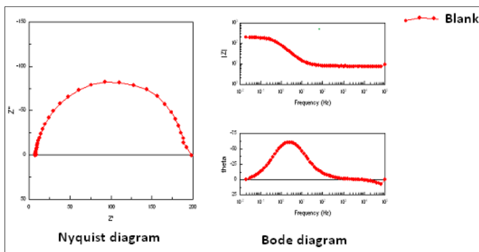
Figure 9. Nyquist and Bode diagrams obtained by EIS of steel immersed in contaminated injection water by 10^2 germs/mL of SRB
