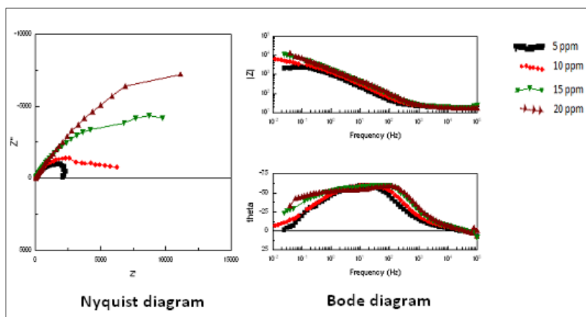
Figure 10. Nyquist and Bode diagrams obtained by EIS of steel immersed in a contaminated injection water by 10^2 germs/mL of SRB and treated with various bio natural product B (5, 10, 15 and 20 ppm)
