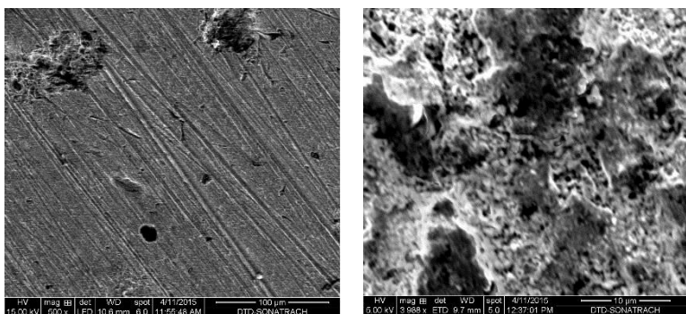
Figure 3. SEM micrographs of steel immersed in contaminated medium by the SRB for 10 days
