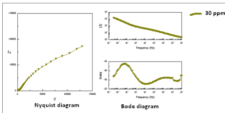
Figure 11. Nyquist and Bode diagrams obtained by EIS of steel immersed in contaminated injection water by 10^2 germs/mL of SRB and treated with 30 ppm of bio natural product B
